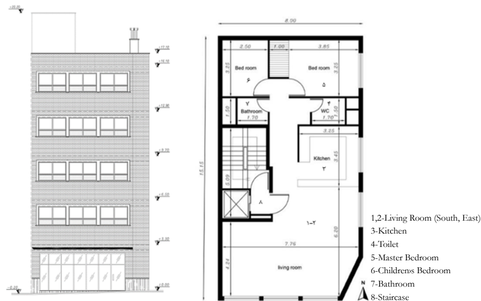
Fig 1: Right: The fifth floor plan and features of the spaces under study, Left: the building facade.
