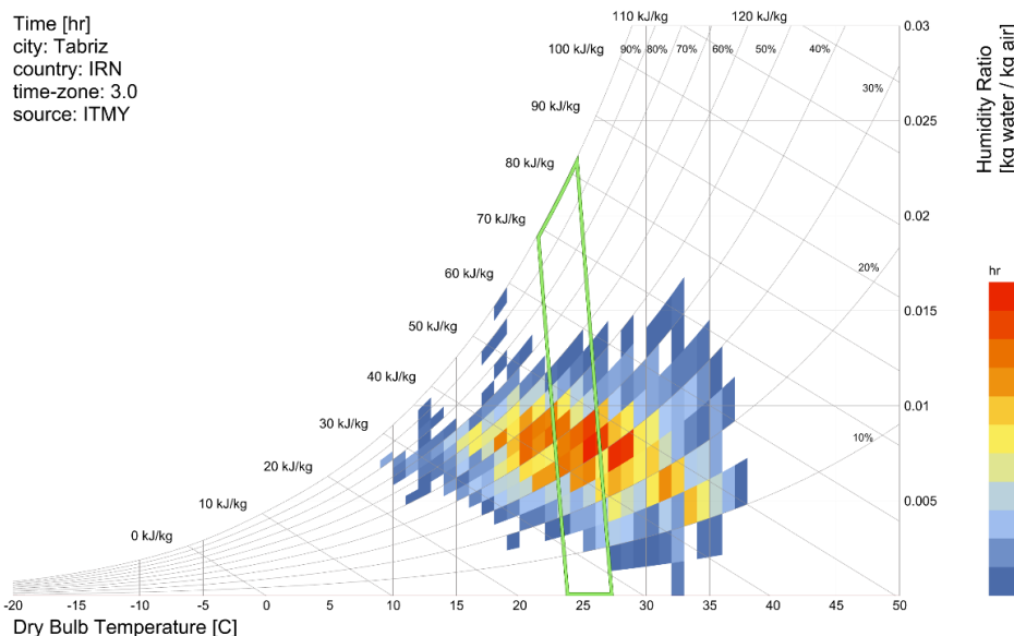
Fig. 3: Tabriz Psychrometric Chart without using any active or passive cooling systems (onebuilding.org)
