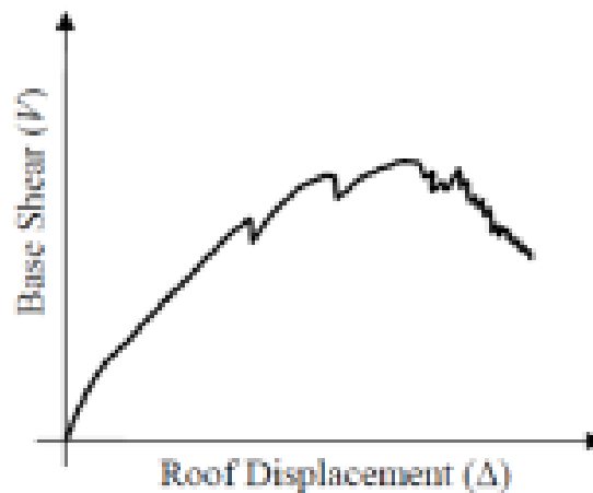
(b) Capacity Curve
