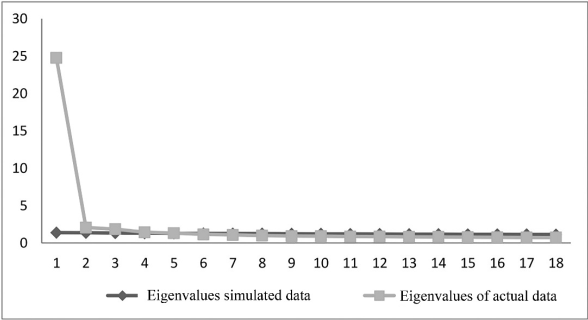
Fig. 1- Scree plots with parallel analysis
