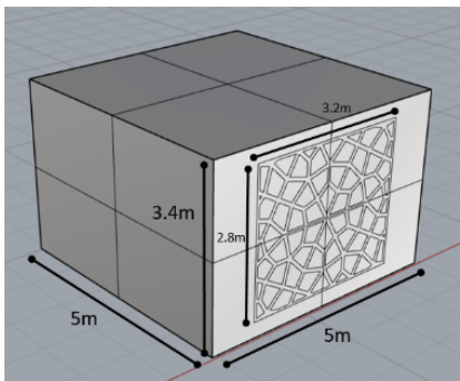
Fig 4. Window and room dimensions of the simulation
